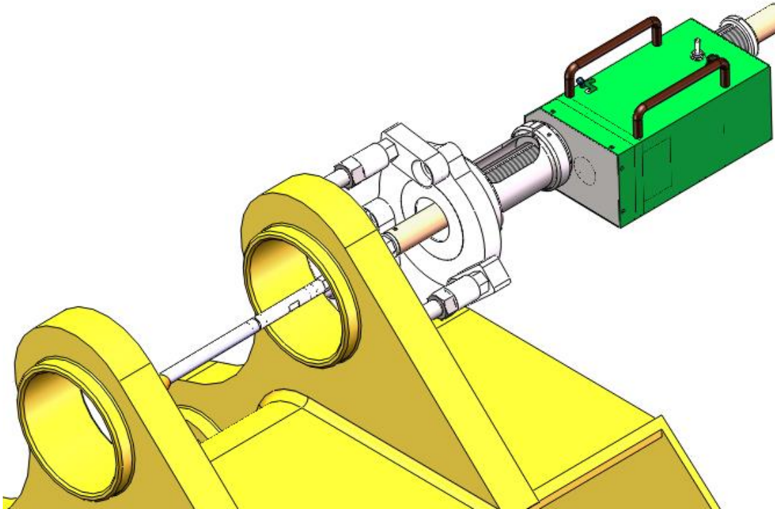
Plan 1: Support tube
